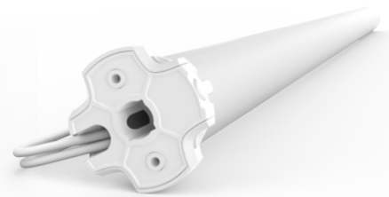
Automate Wire-Free Li-ion Q10 12V, 10.0Nm, Ø45mm, 9-5RPM, 32.04in long
