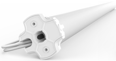
Automate Wire-Free Li-ion 3.0 12V, 3.0Nm, Ø35mm, 20-28PRM, 33.41in long
