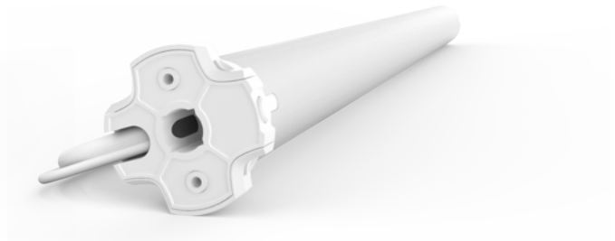
Automate ACRF Q6 110-120 A/C, 6.0Nm, Ø35mm, 24RPM, 21.18in long
